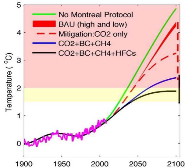
Fig. 3: 21 st Century warming prevented by SLCP and CO 2 mitigation
